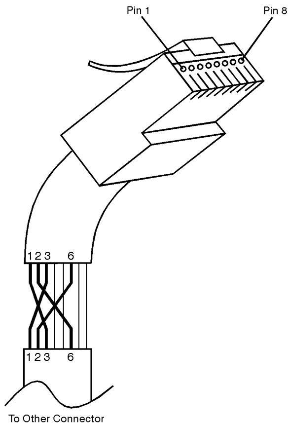
Figure 6-2 Cross-Over Patch Cable Wiring (cross-over end)
